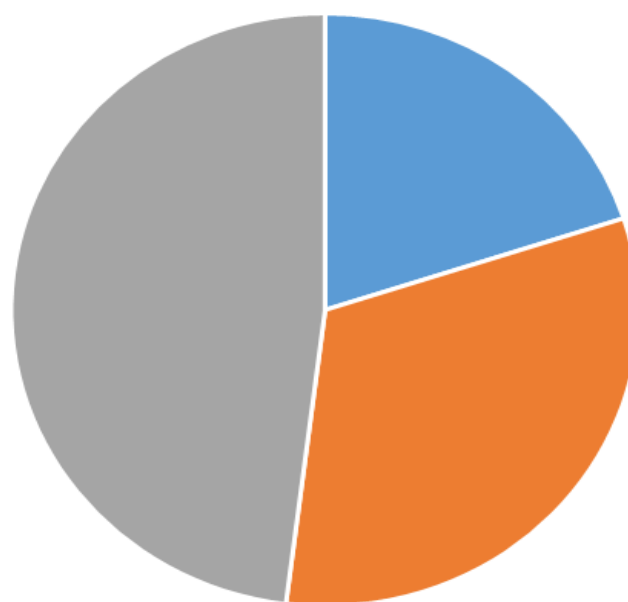
Figure 6.3: Residue in Wildcat Creek
